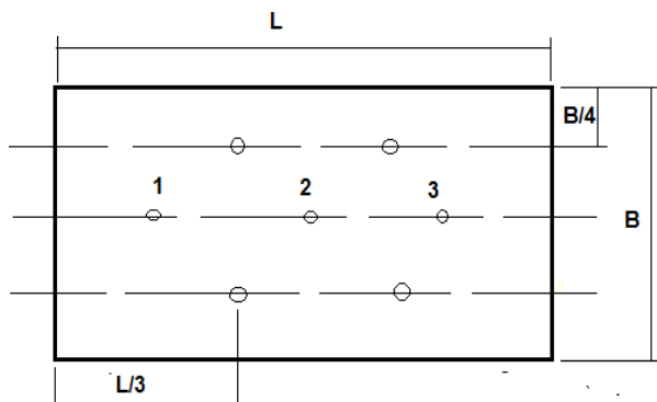
Figure 3.3.7.3 Measurements of 7 thicknesses fore and aft on a plate
